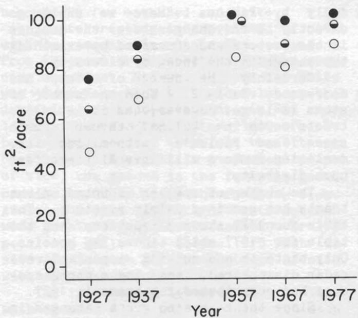
Fig. 5. The basal area of major species (ft 2 /acre) on moist (●), medium (◐) and dry (○) sites.
