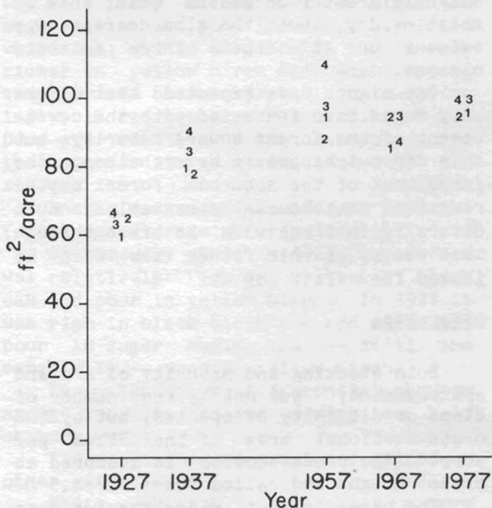
Fig. 7. The basal area (ft 2 /acre) of major species on Cox (1), Turkey Hill (2), Reeves (3), and Cabin (4) tracts.
