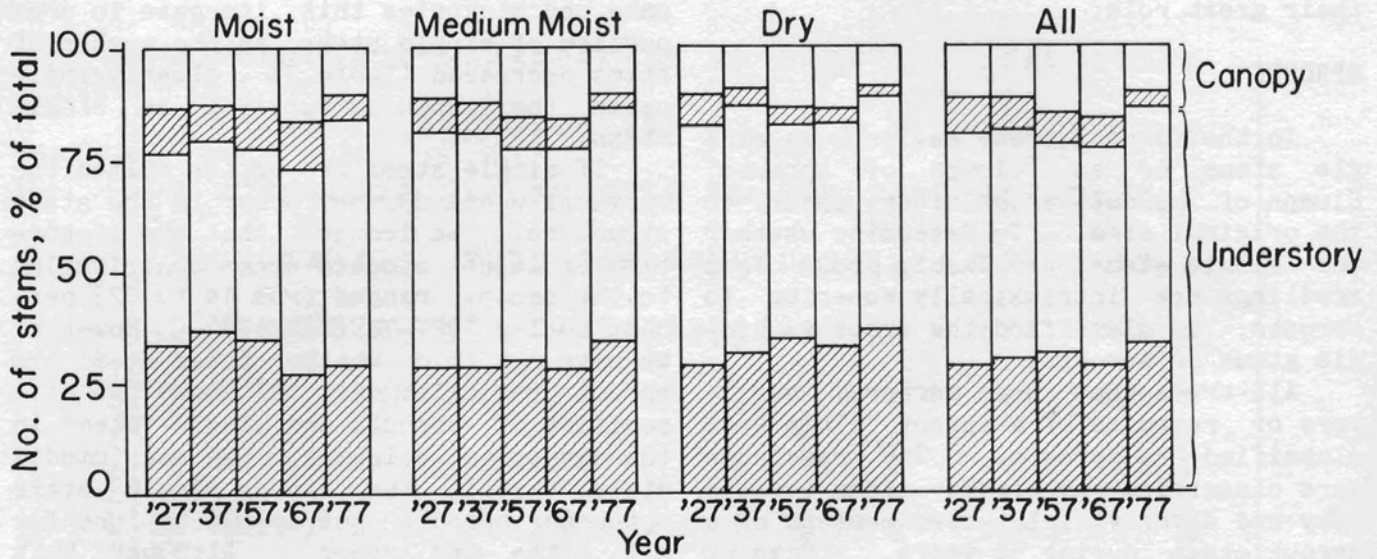
Fig. 11. Distribution of single stems \square and sprouts \text{▨} of major species in the canopy (percent), all tracts. Upper: dominant and codominant trees in the canopy; lower: intermediate and overtopped stems beneath the canopy. All moisture classes includes trees on muck.
