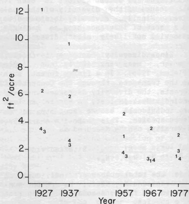
Fig. 8. The basal area (ft 2 /acre) of minor species on Cox (1), Turkey Hill (2), Reeves (3), and Cabin (4) tracts.
