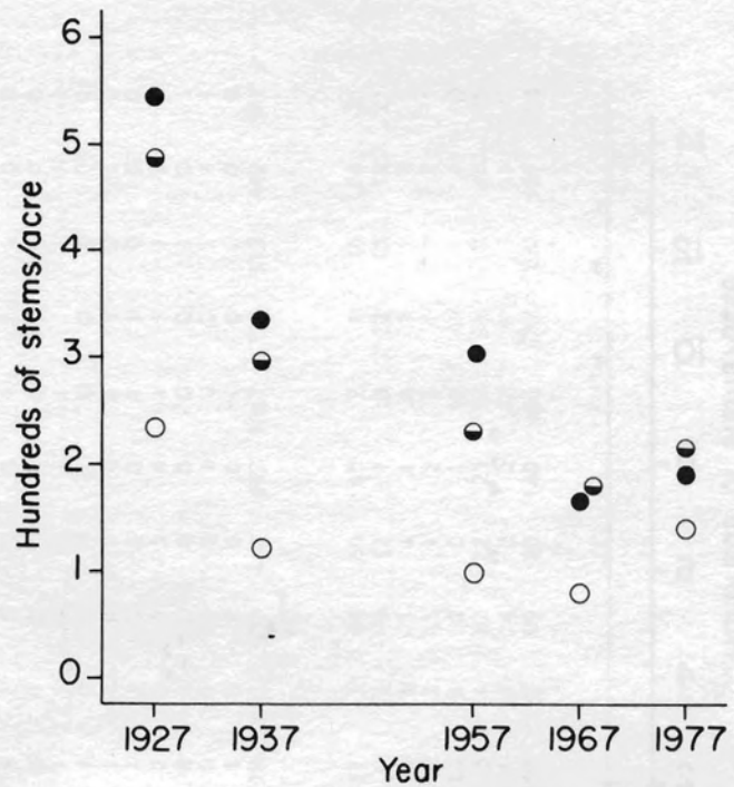
Fig. 2. The number of minor species stems per acre on moist (●), medium (◐) and dry (○) sites.
