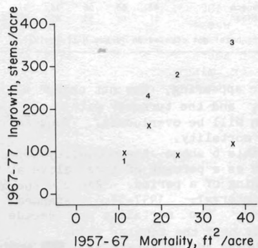
Fig. 10. The ingrowth of major (numbered) and minor (X) species on four tracts during 1967-77 as a function of the mortality of basal area during the preceding decade. Turkey Hill (1), Cox (2), Reeves (3), Cabin (4).
