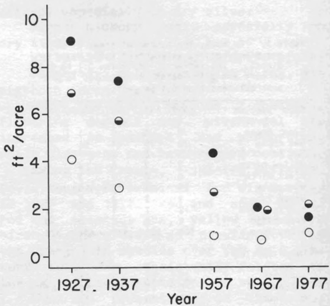
Fig. 6. The basal area of minor species (ft 2 /acre) on moist (●), medium (◐) and dry (○) sites.
