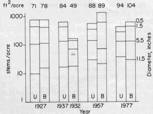
Fig. 12. The Turkey Hill forest that was unburned (U) and burned (B) in 1932. On a logarithmic scale, the numbers of stems/acre with diameter greater than 0.5, 1.5, 5.5 and 11.5 inches. At the top of the graph are shown basal areas of stems in \text{ft}^2/\text{acre} .
